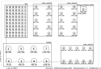
Component layout diagram
