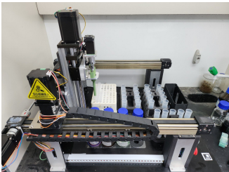
Automated Mixing Device (MolGeniusComposer)
